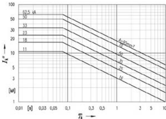
Fig. 2: Admissible current carrying capacity of short circuit cables made of Cu for use in d.c.installations
