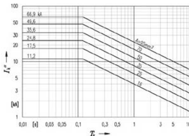
Fig. 3: Admissible current carrying capacity of short circuit cables made of Cu for use on overhead contact wires on electric railways
