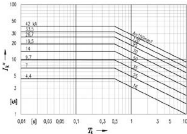
Fig. 1: Admissible current carrying capacity of short circuit cables made of Cu for use in installations with alternating and 3-phase current
