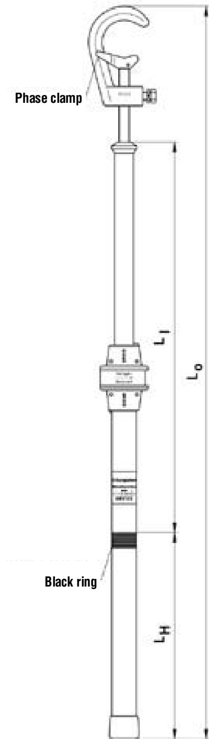
Fig. 1: Telescopic earthing rod
